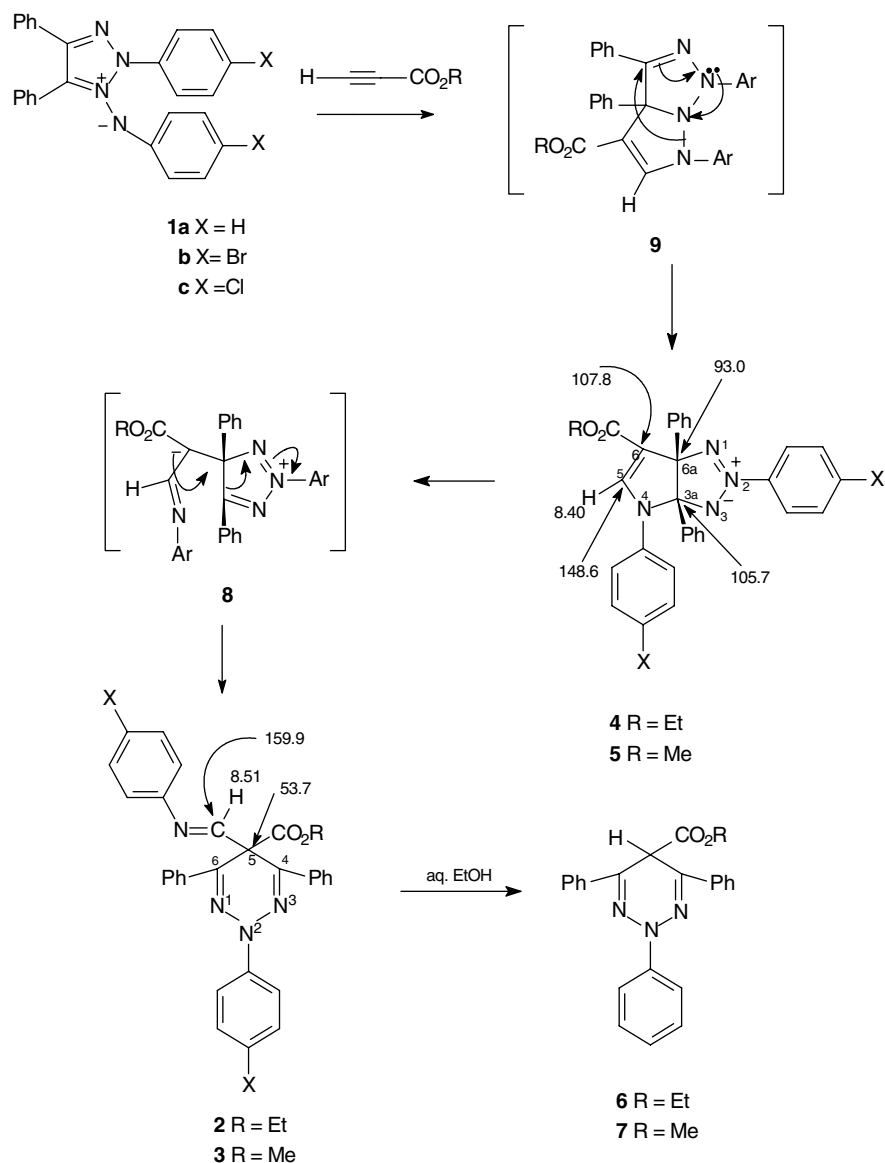
Scheme 1. ^1\text{H} and ^{13}\text{C} NMR shifts in \text{CDCl}_3 for 2a and 4a .
