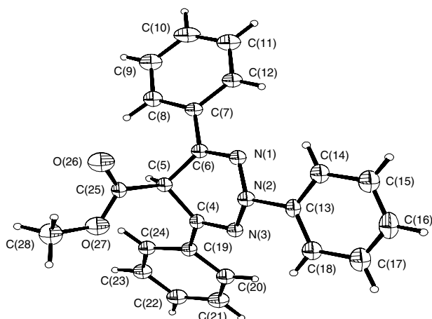
Figure 3. X-ray crystal structure of 7 .
